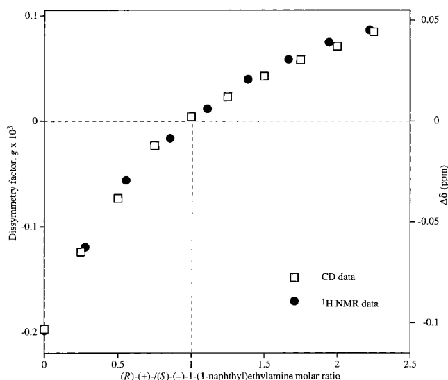
Figure 8. Changes of the dissymmetry factor ( g ) at the wavelength corresponding to the maximum of the first Cotton effect and B_{II} band, and the corrected chemical shift difference ( \Delta\delta ) between 10- and 20- meso protons of the bis(Zn porphyrin):(R)-(+)-1-(1-naphthyl)ethylamine mixture upon titration with (S)-(-)-1-(1-naphthyl)ethylamine.
