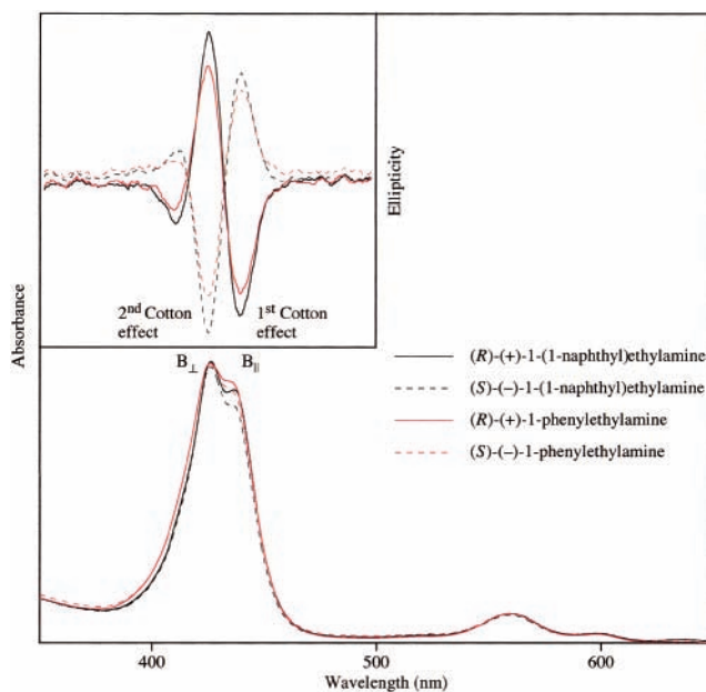
Figure 3. Static UV-vis and CD (inset) spectra of bis(Zn porphyrin) in \text{CH}_2\text{Cl}_2 containing different chiral amines at 293 K; C_{\text{bis(Zn porphyrin)}} = (3.1\text{--}3.4) \times 10^{-6} M, C_{\text{amine}} = (4.1\text{--}5.1) \times 10^{-2} M.
